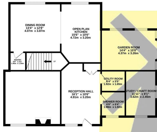
GROUND FLOOR 1089 sq.ft. (101.2 sq.m.) approx.
